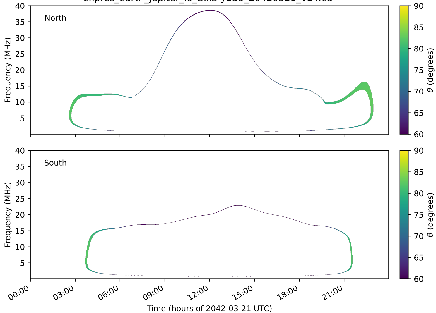
expres_earth_jupiter_io_txka-y235_20420321_v14.cdf
