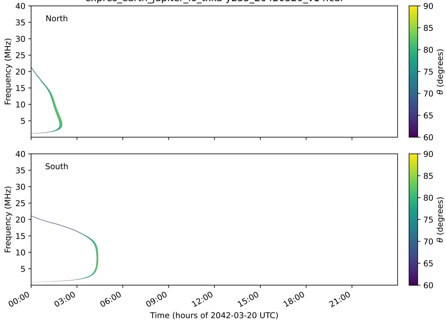
expres_earth_jupiter_io_txka-y235_20420320_v14.cdf
