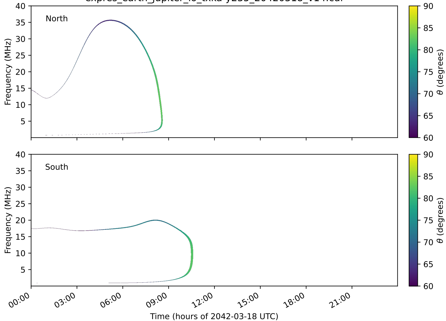
expres_earth_jupiter_io_txka-y235_20420318_v14.cdf
