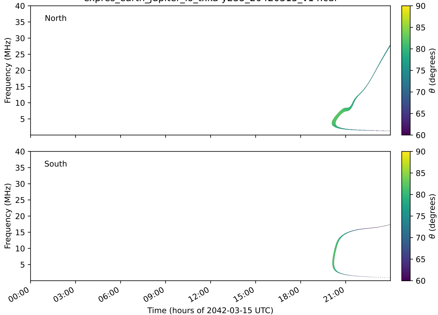
expres_earth_jupiter_io_txka-y235_20420315_v14.cdf
