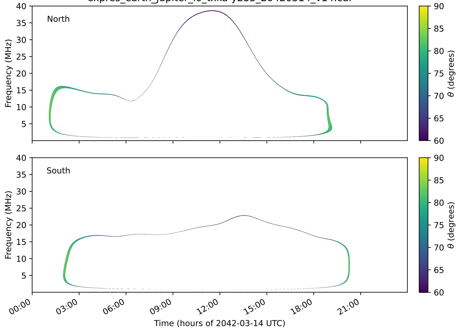
expres_earth_jupiter_io_txka-y235_20420314_v14.cdf
