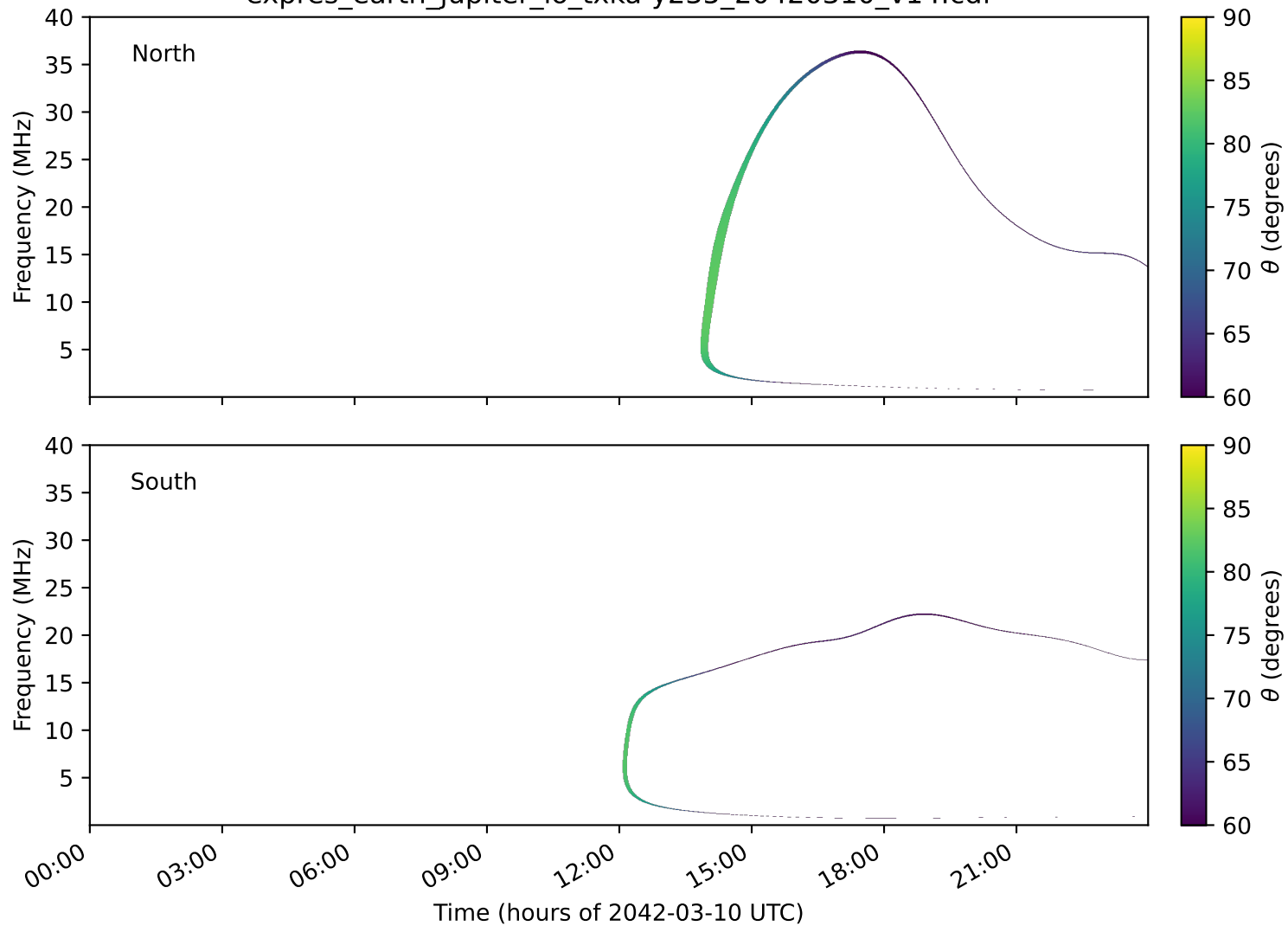
expres_earth_jupiter_io_txka-y235_20420310_v14.cdf
