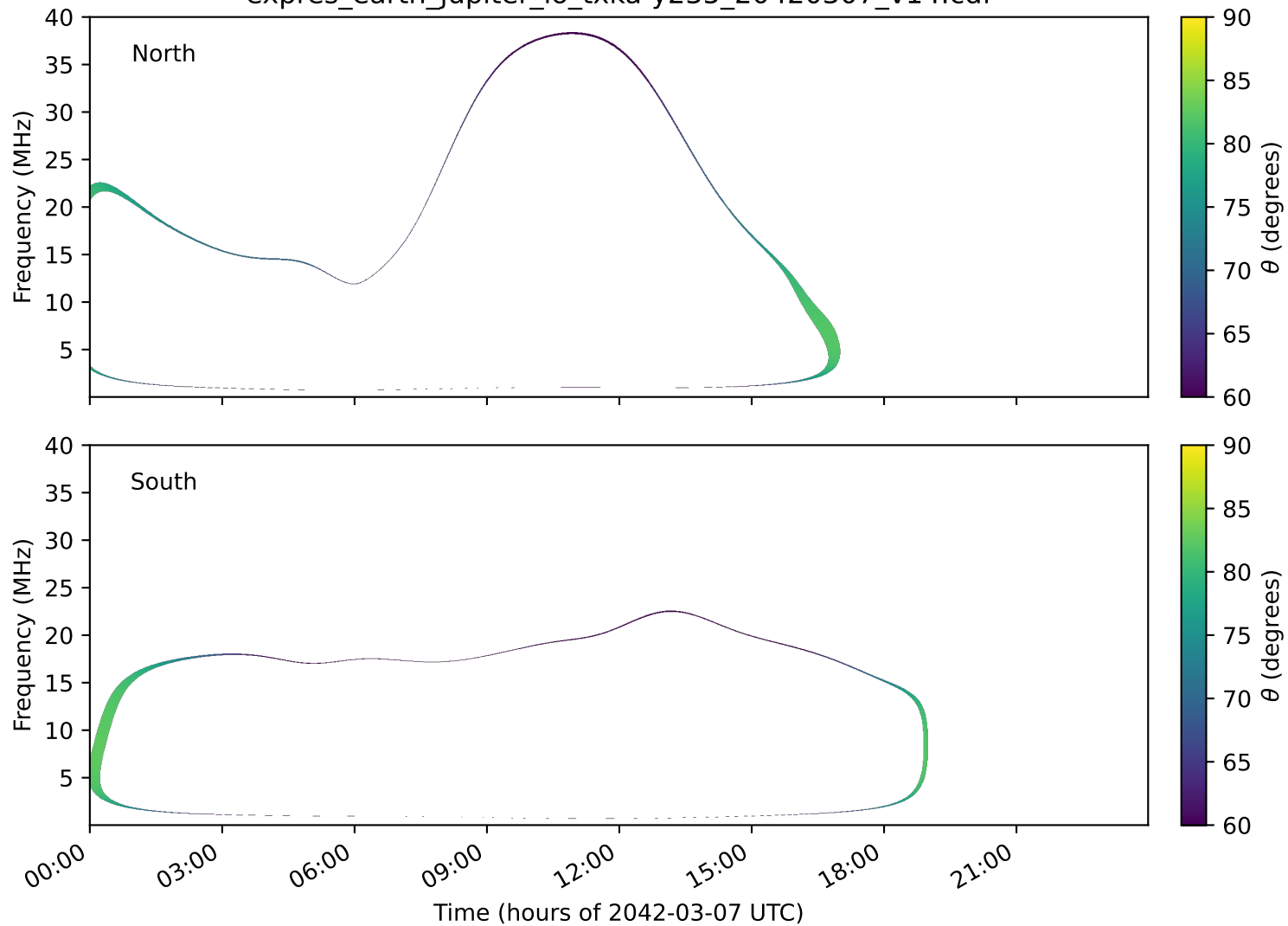
expres_earth_jupiter_io_txka-y235_20420307_v14.cdf
