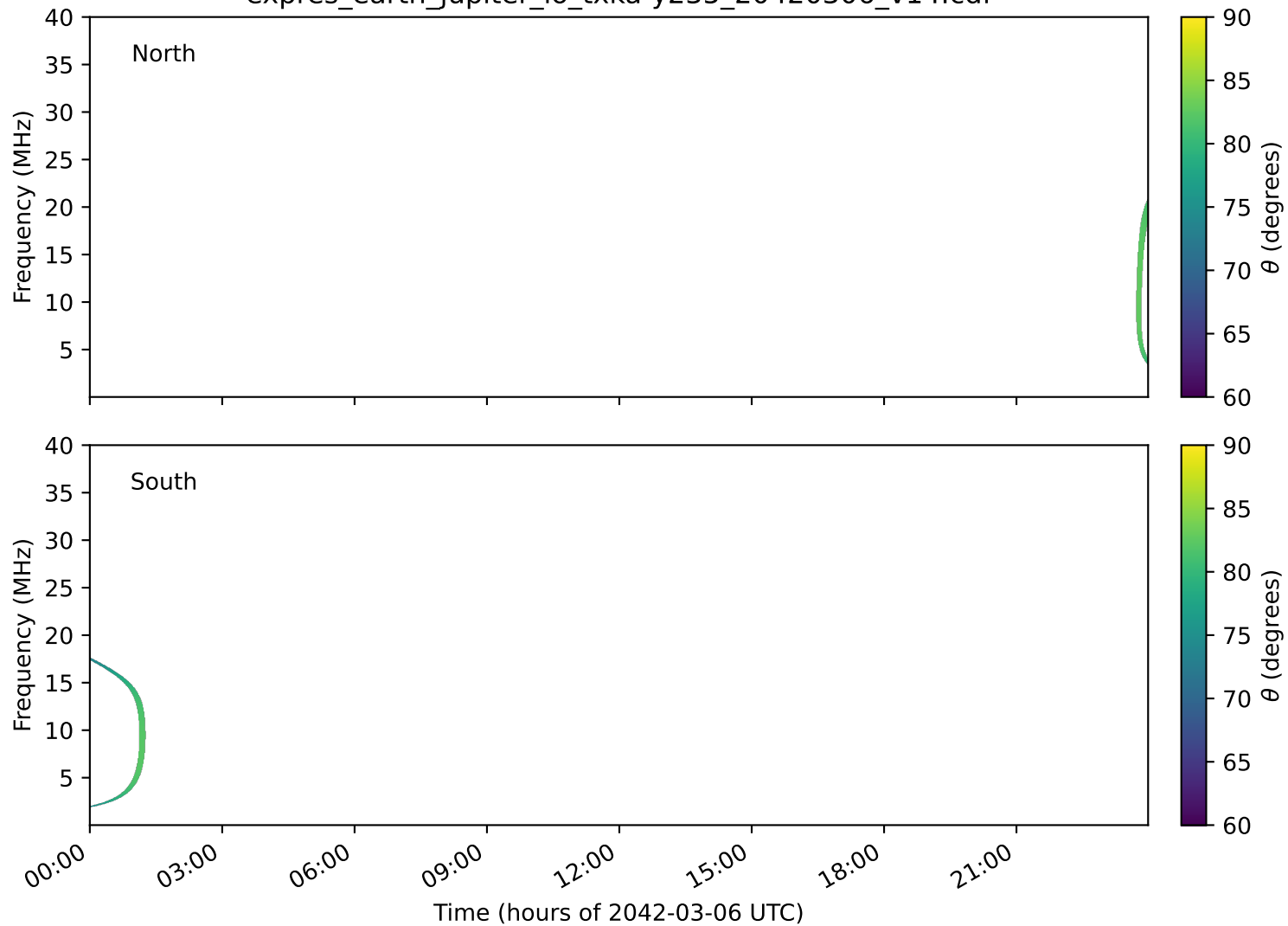
expres_earth_jupiter_io_txka-y235_20420306_v14.cdf
