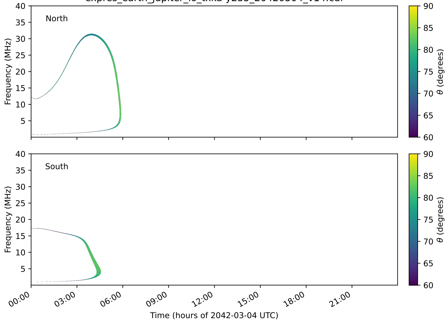
expres_earth_jupiter_io_txka-y235_20420304_v14.cdf
