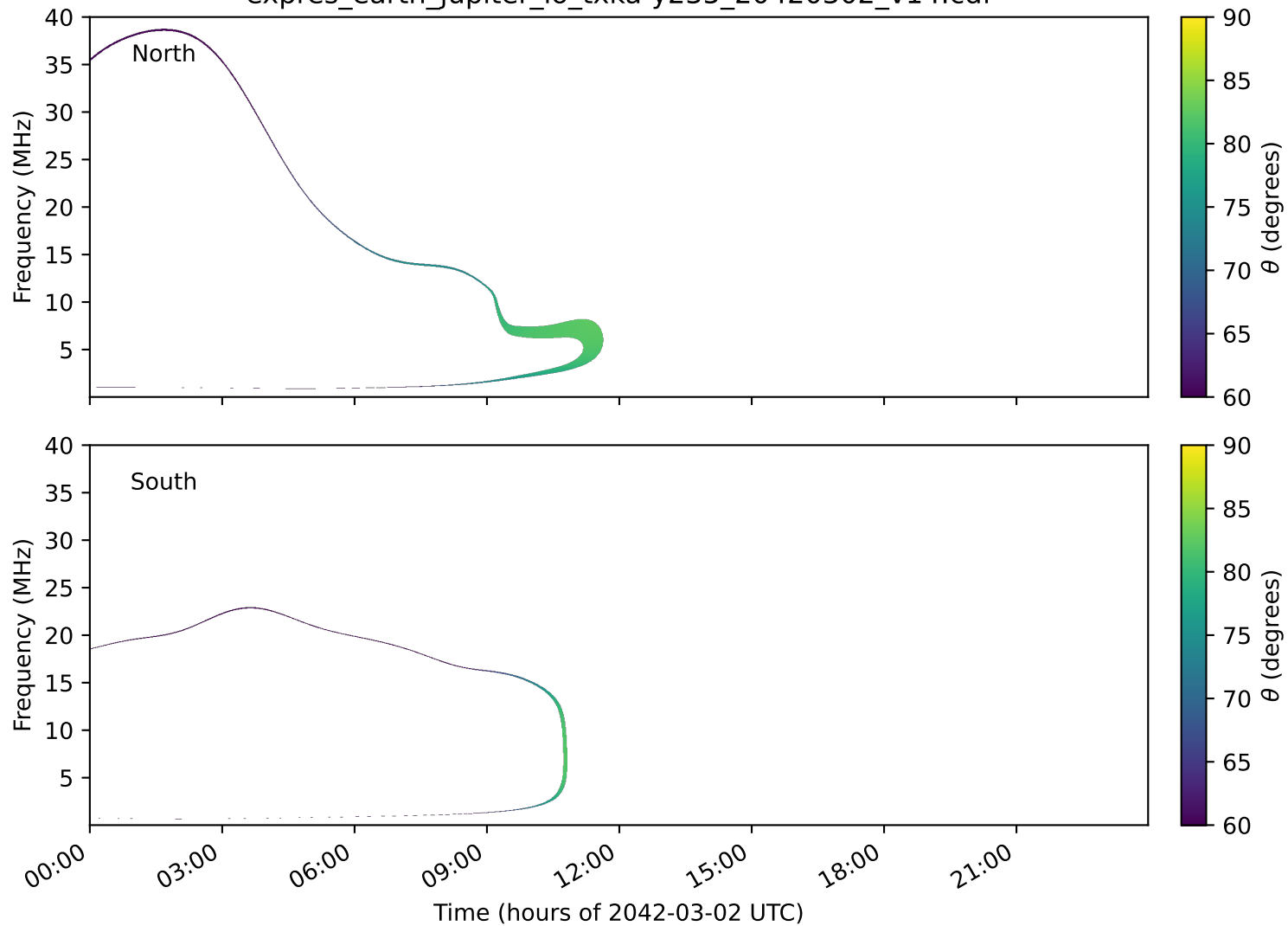
expres_earth_jupiter_io_txka-y235_20420302_v14.cdf
