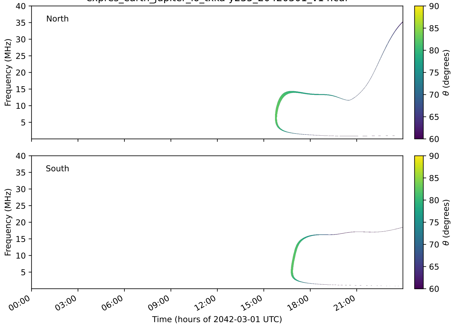
expres_earth_jupiter_io_txka-y235_20420301_v14.cdf
