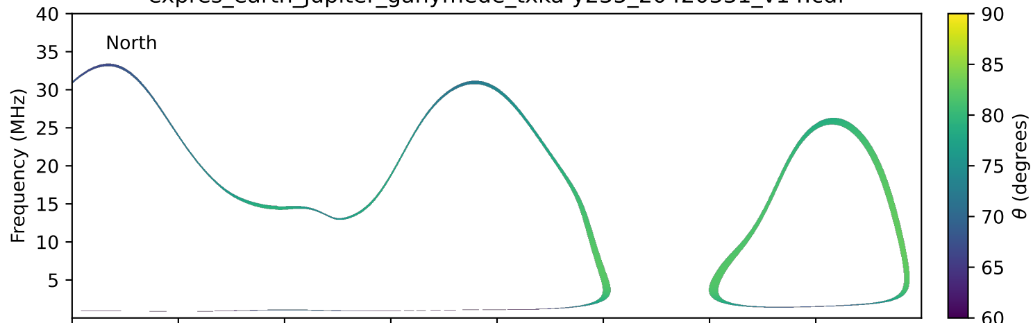
expres_earth_jupiter_ganymede_txka-y235_20420331_v14.cdf
