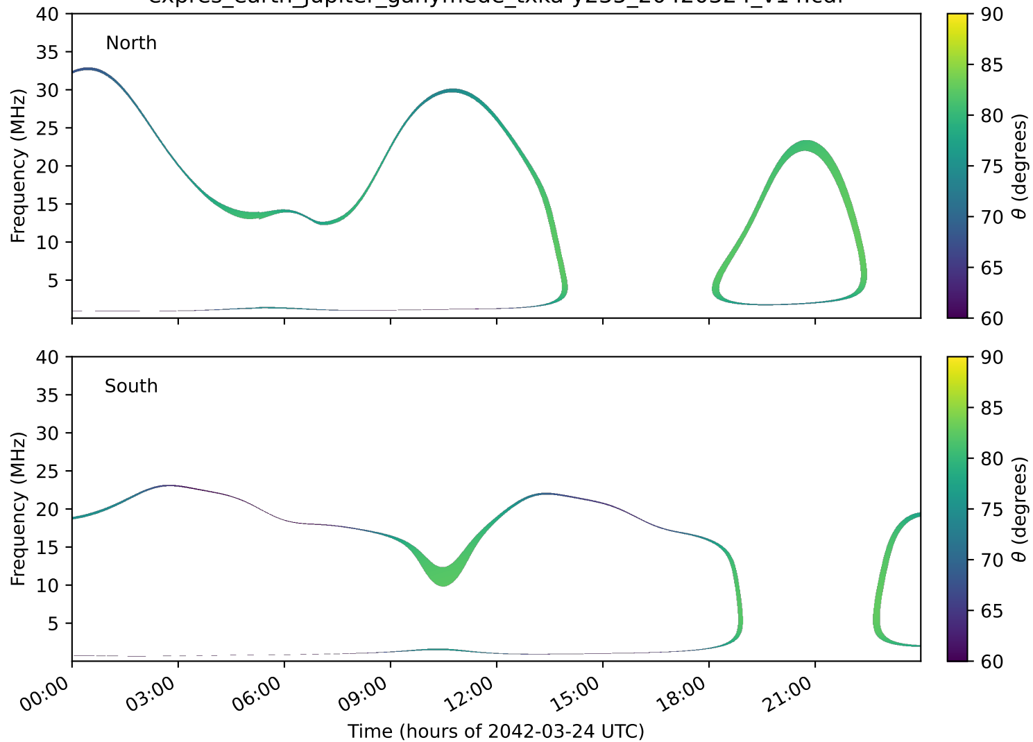
expres_earth_jupiter_ganymede_txka-y235_20420324_v14.cdf
