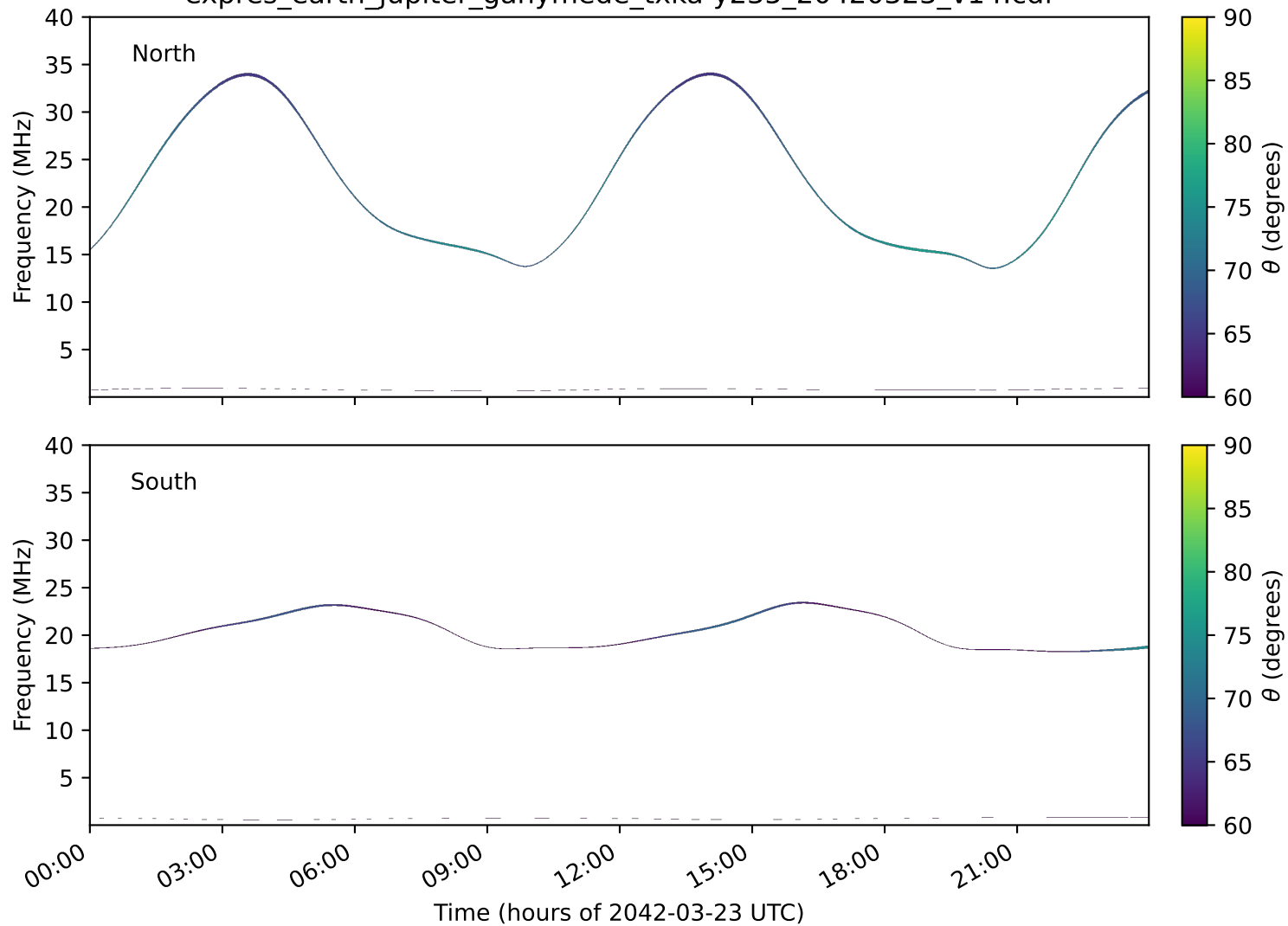
expres_earth_jupiter_ganymede_txka-y235_20420323_v14.cdf
