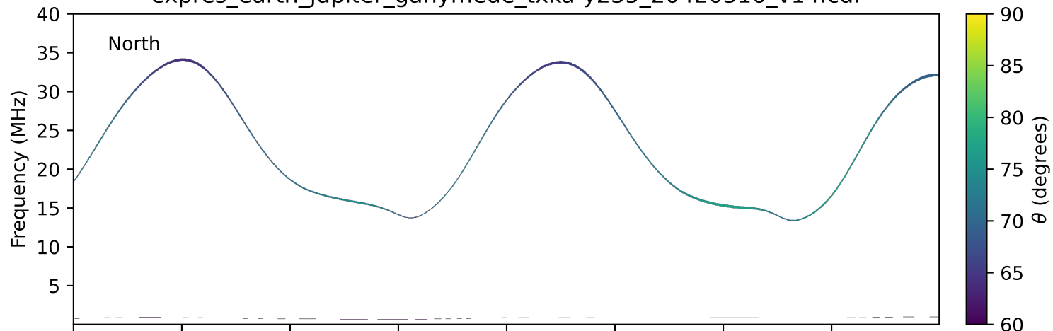
expres_earth_jupiter_ganymede_txka-y235_20420316_v14.cdf
