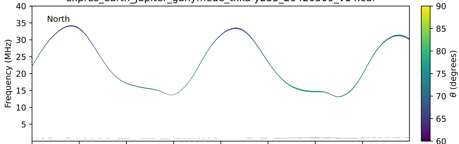
expres_earth_jupiter_ganymede_txka-y235_20420309_v14.cdf
