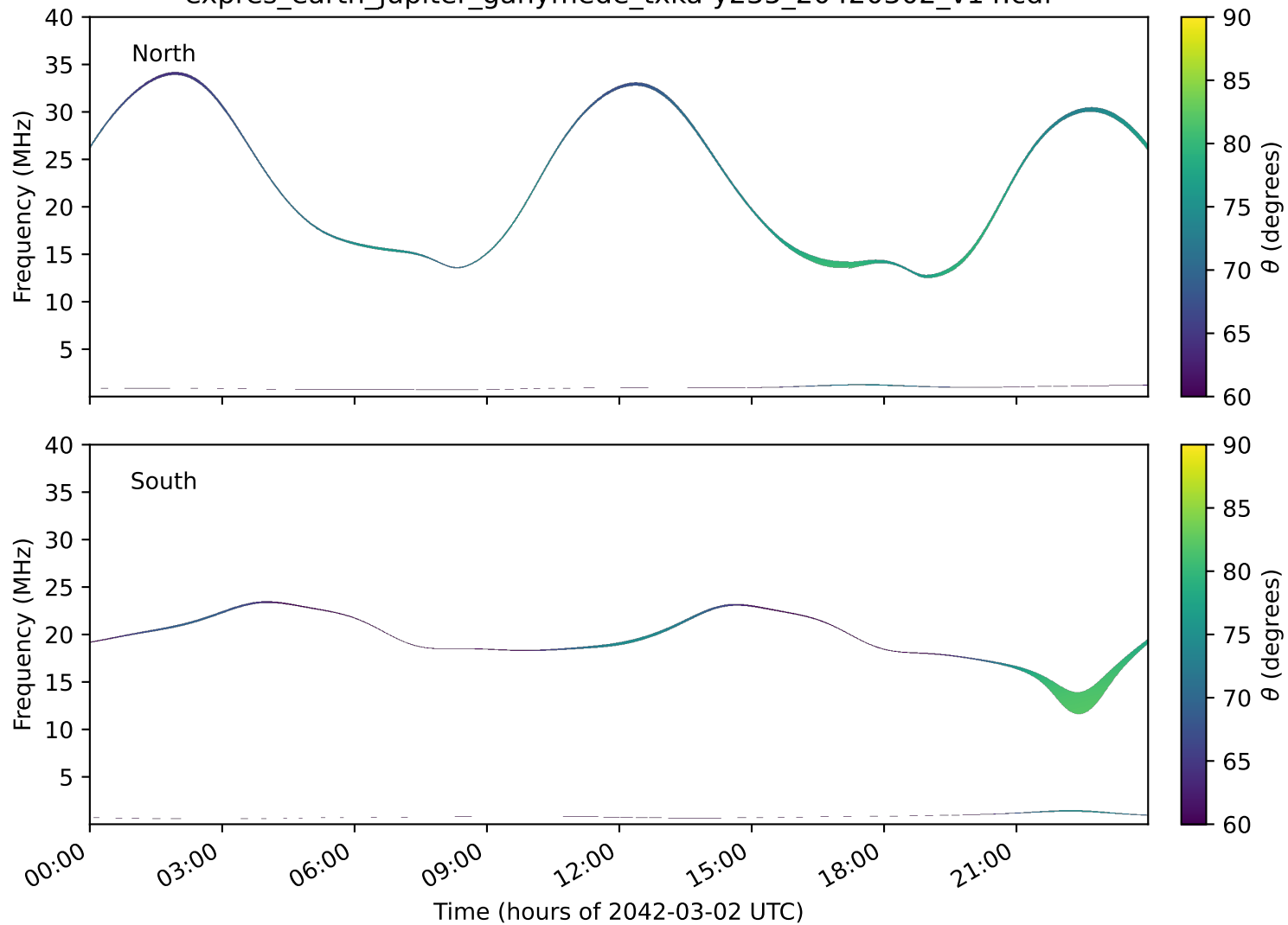
expres_earth_jupiter_ganymede_txka-y235_20420302_v14.cdf
