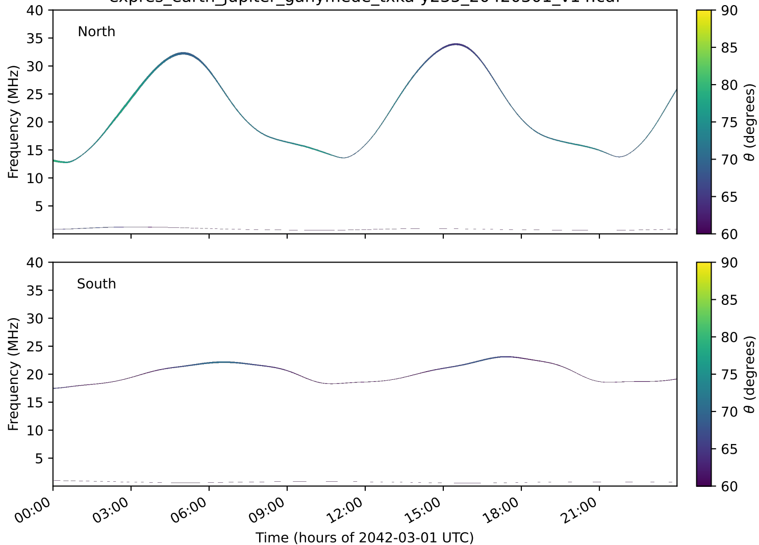
expres_earth_jupiter_ganymede_txka-y235_20420301_v14.cdf
