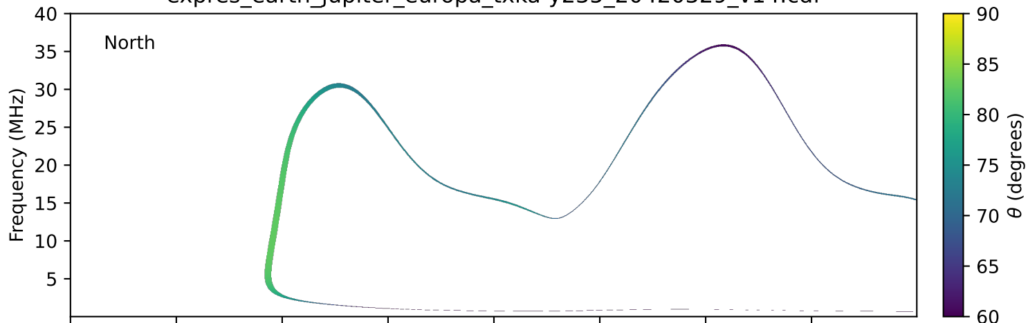
expres_earth_jupiter_europa_txka-y235_20420329_v14.cdf
