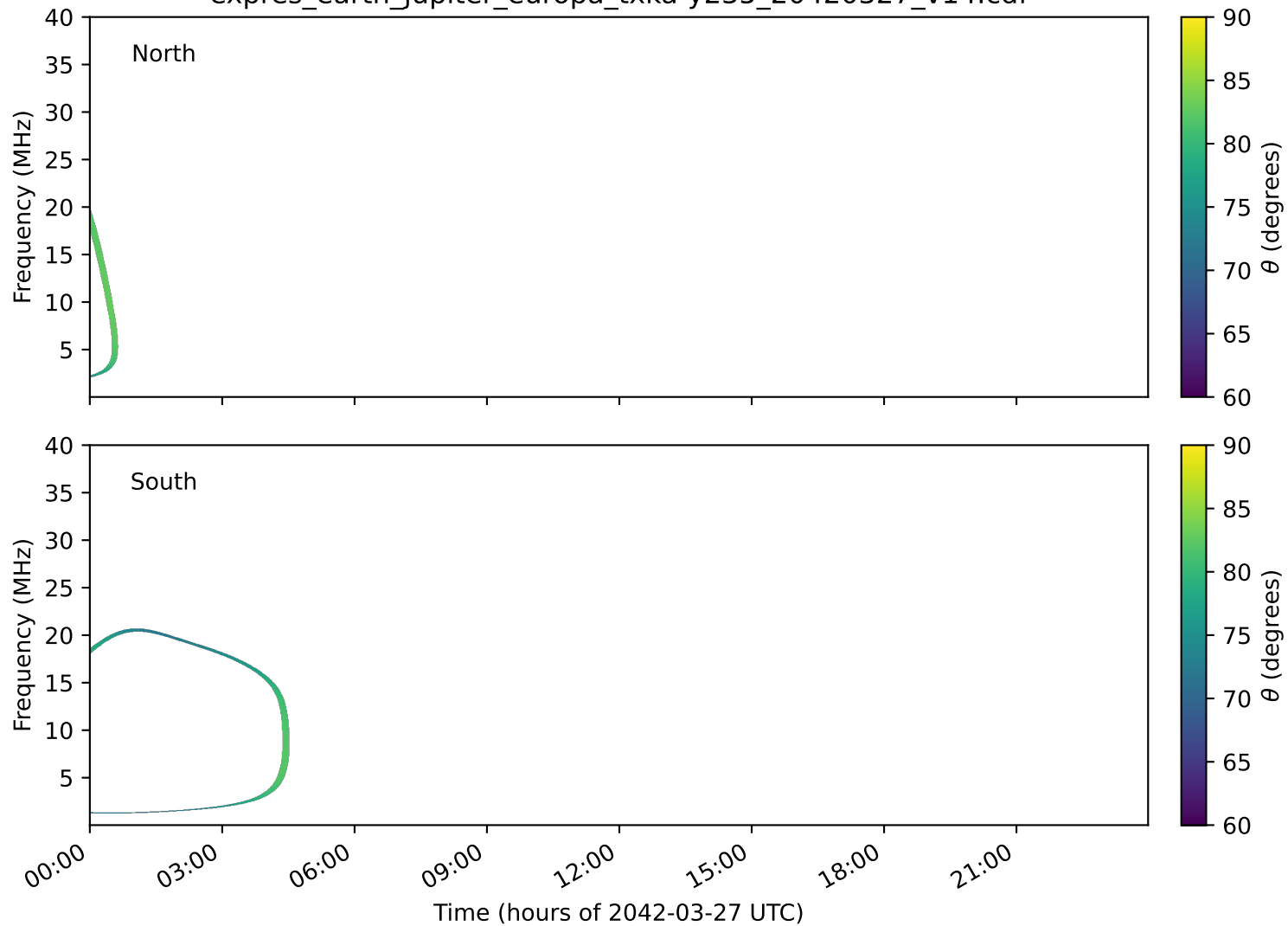
expres_earth_jupiter_europa_txka-y235_20420327_v14.cdf
