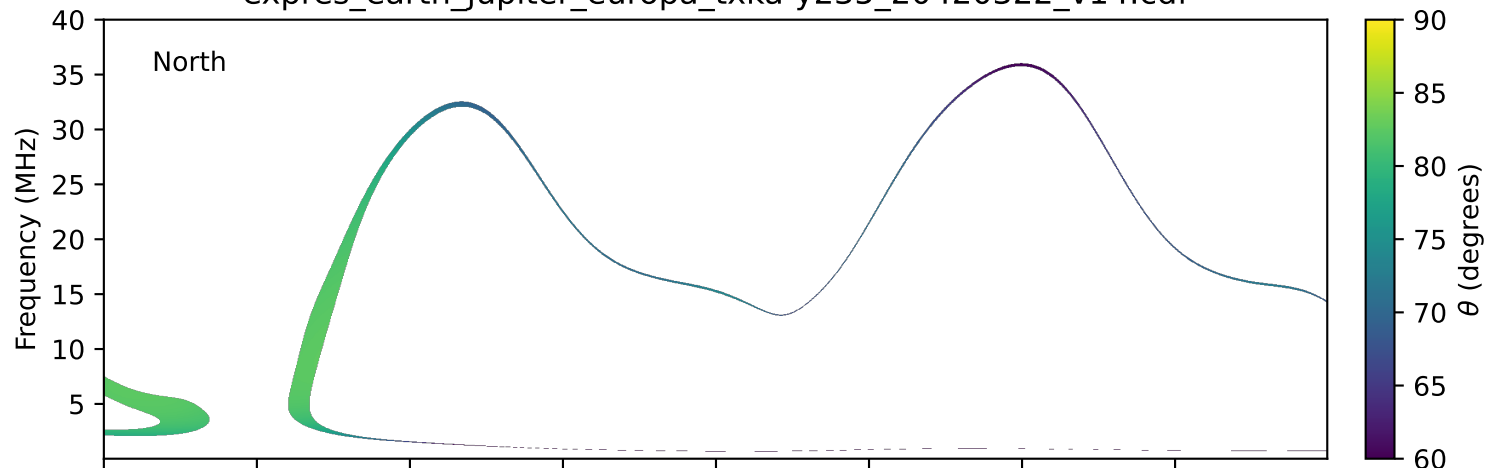
expres_earth_jupiter_europa_txka-y235_20420322_v14.cdf
