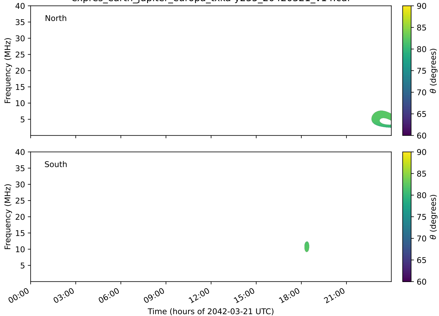
expres_earth_jupiter_europa_txka-y235_20420321_v14.cdf
