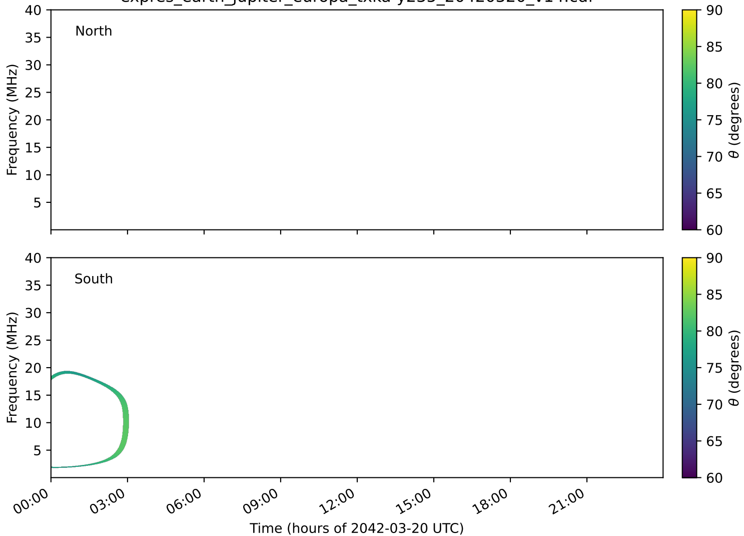
expres_earth_jupiter_europa_txka-y235_20420320_v14.cdf
