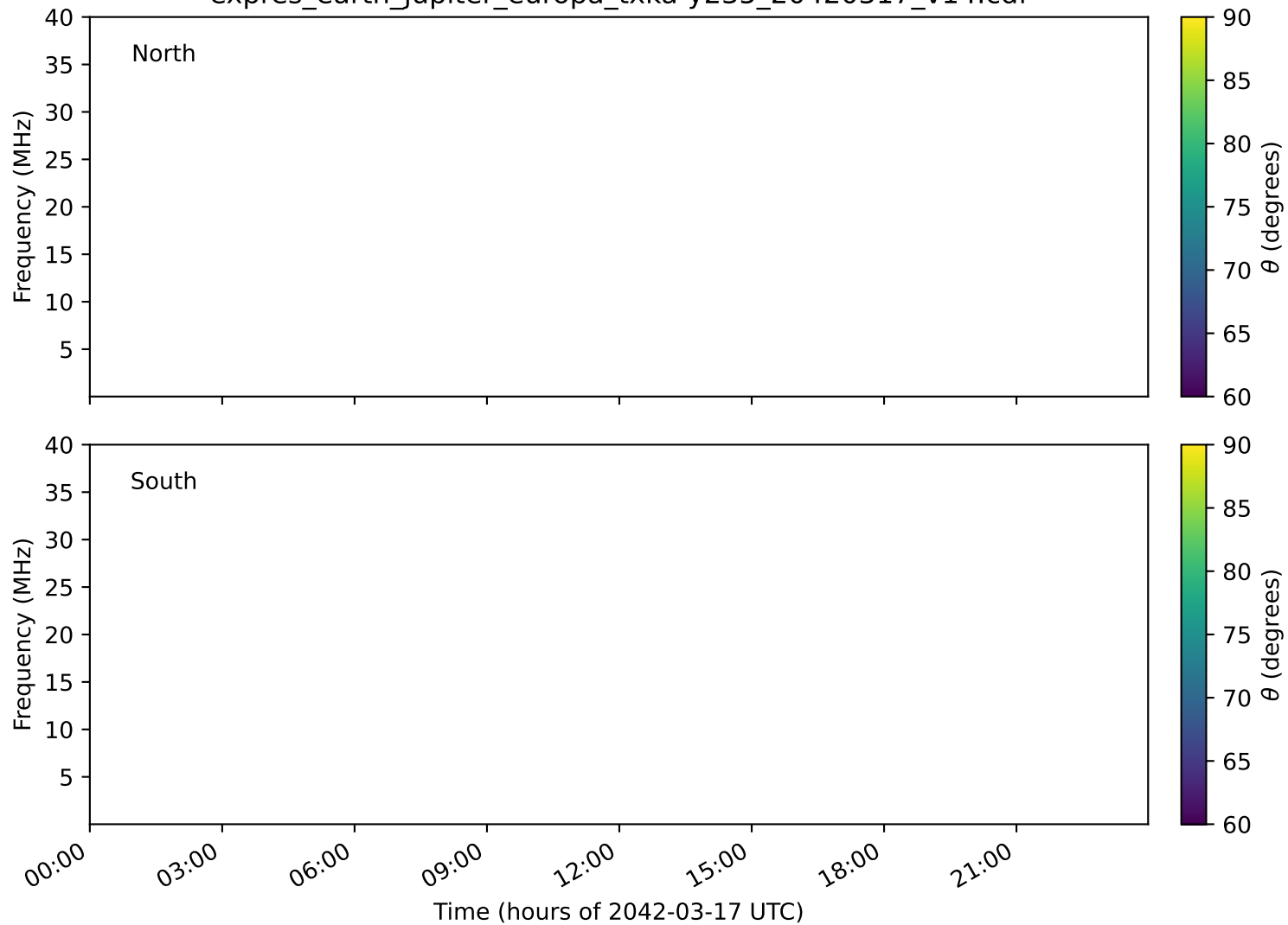
expres_earth_jupiter_europa_txka-y235_20420317_v14.cdf
