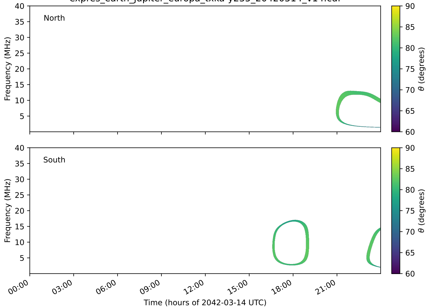
expres_earth_jupiter_europa_txka-y235_20420314_v14.cdf
