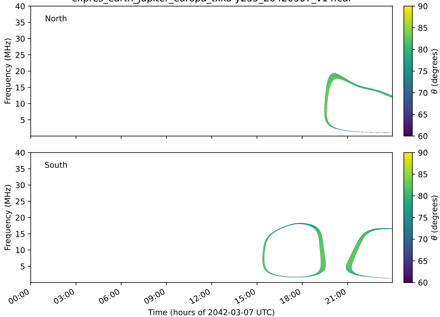
expres_earth_jupiter_europa_txka-y235_20420307_v14.cdf
