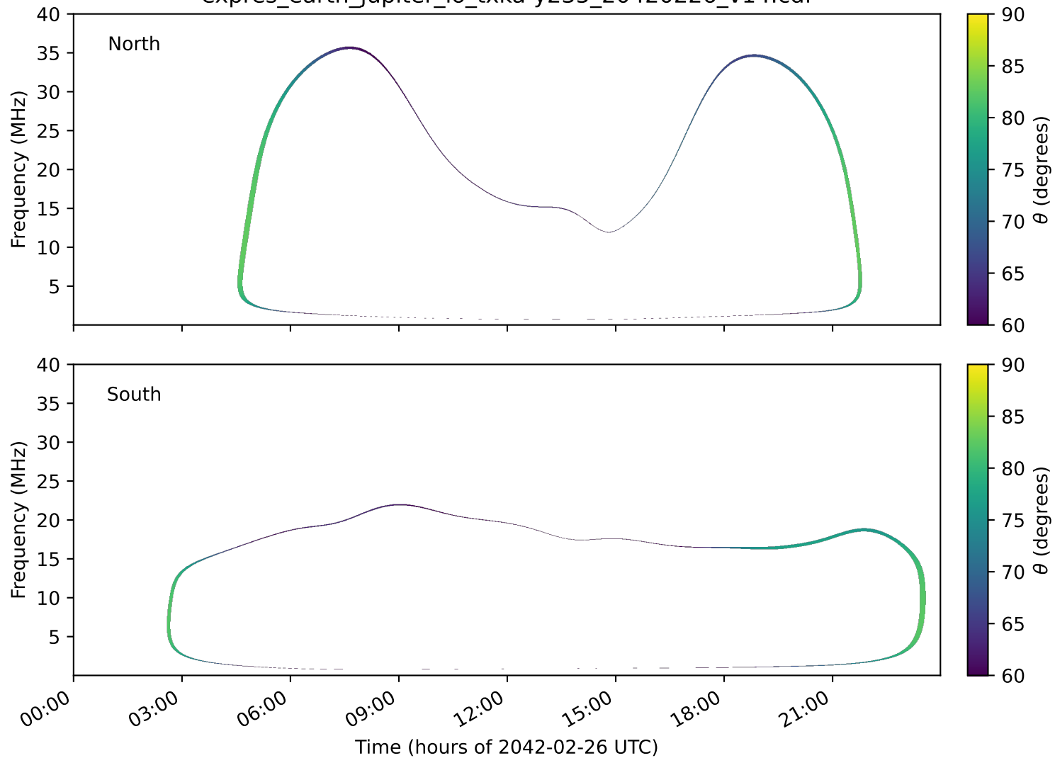
expres_earth_jupiter_io_txka-y235_20420226_v14.cdf
