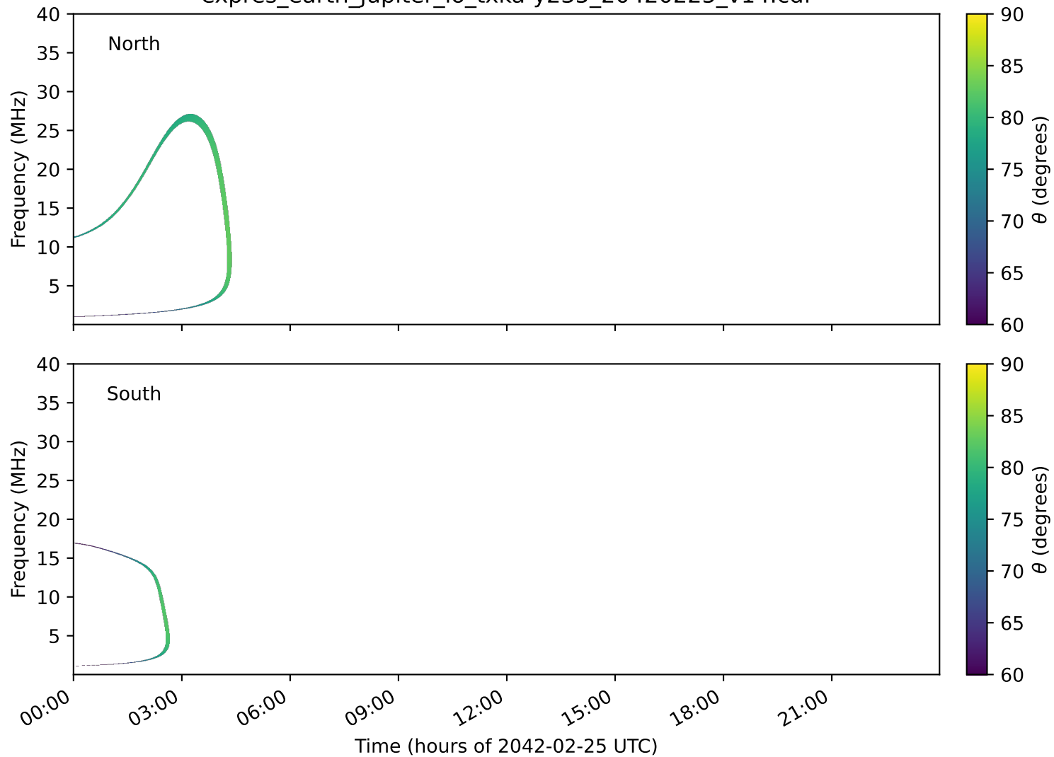
expres_earth_jupiter_io_txka-y235_20420225_v14.cdf
