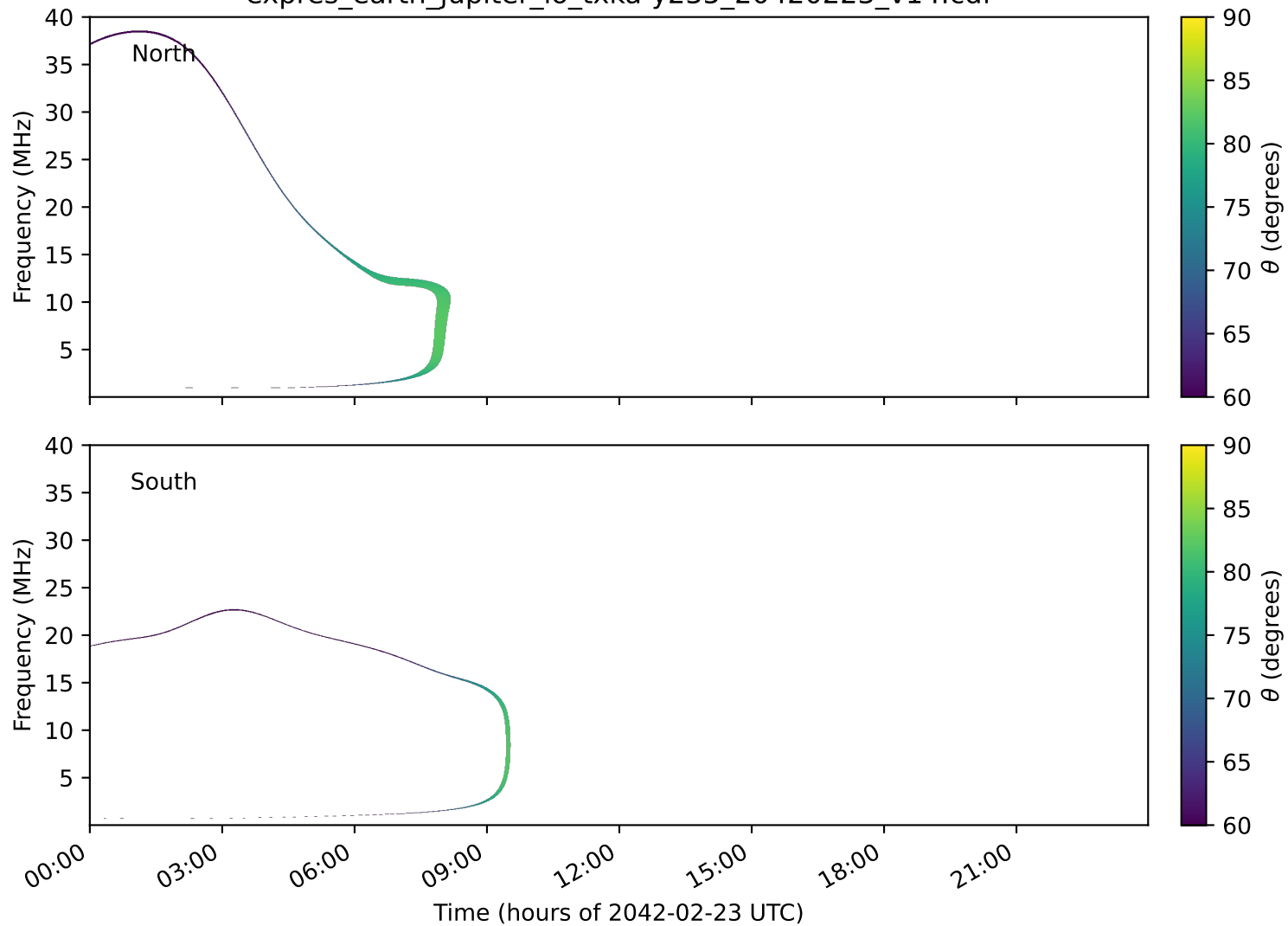
expres_earth_jupiter_io_txka-y235_20420223_v14.cdf
