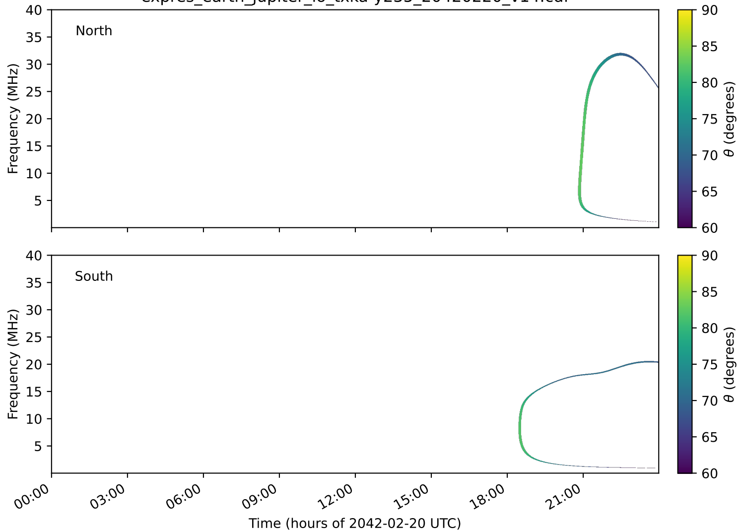
expres_earth_jupiter_io_txka-y235_20420220_v14.cdf
