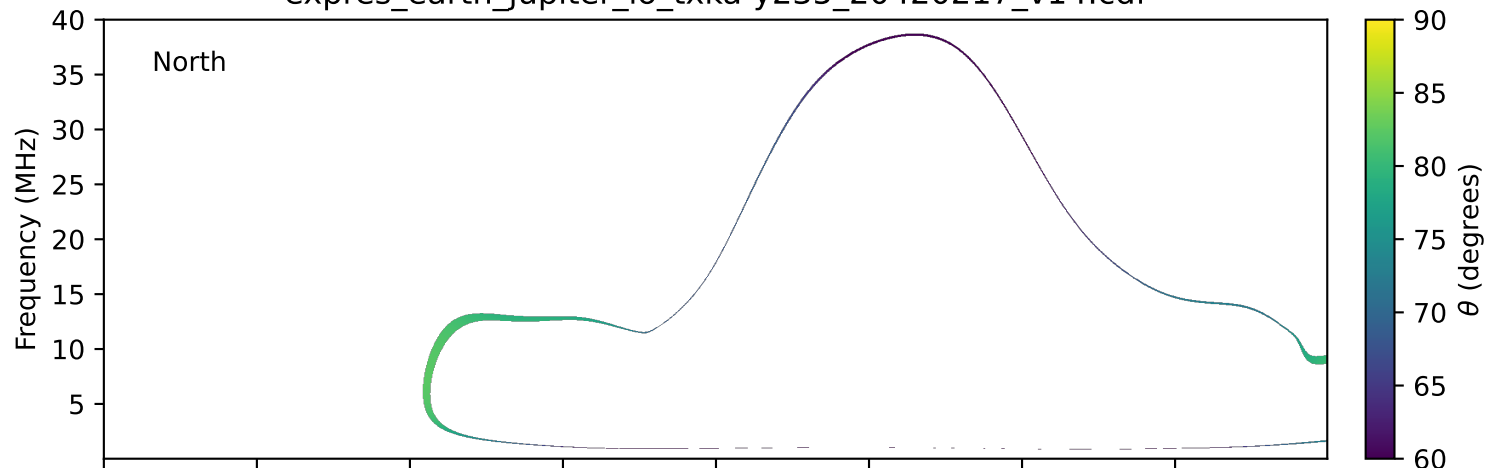
expres_earth_jupiter_io_txka-y235_20420217_v14.cdf
