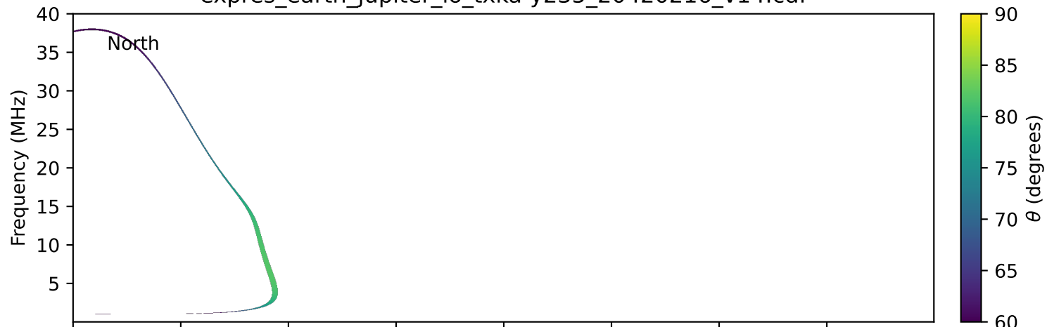
expres_earth_jupiter_io_txka-y235_20420216_v14.cdf
