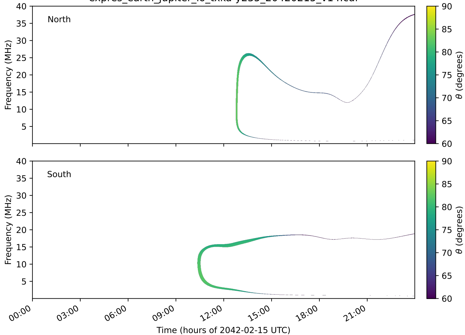
expres_earth_jupiter_io_txka-y235_20420215_v14.cdf
