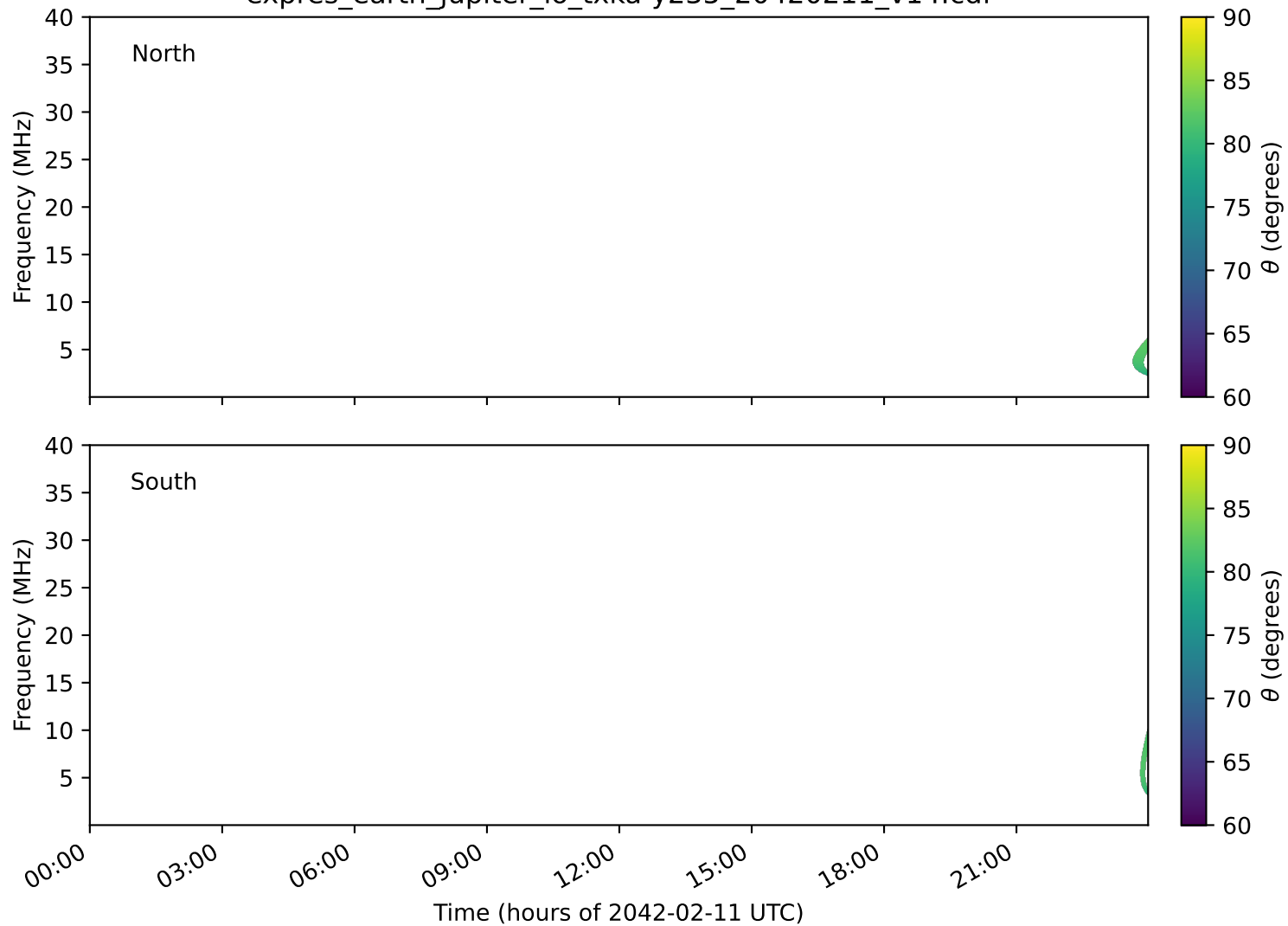
expres_earth_jupiter_io_txka-y235_20420211_v14.cdf
