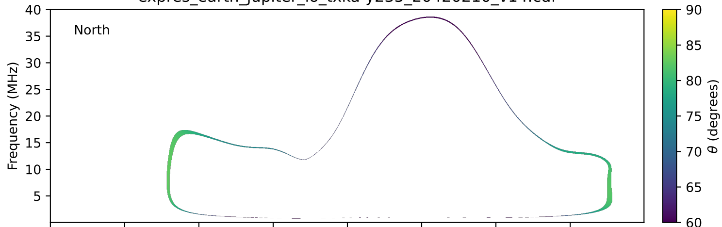
expres_earth_jupiter_io_txka-y235_20420210_v14.cdf
