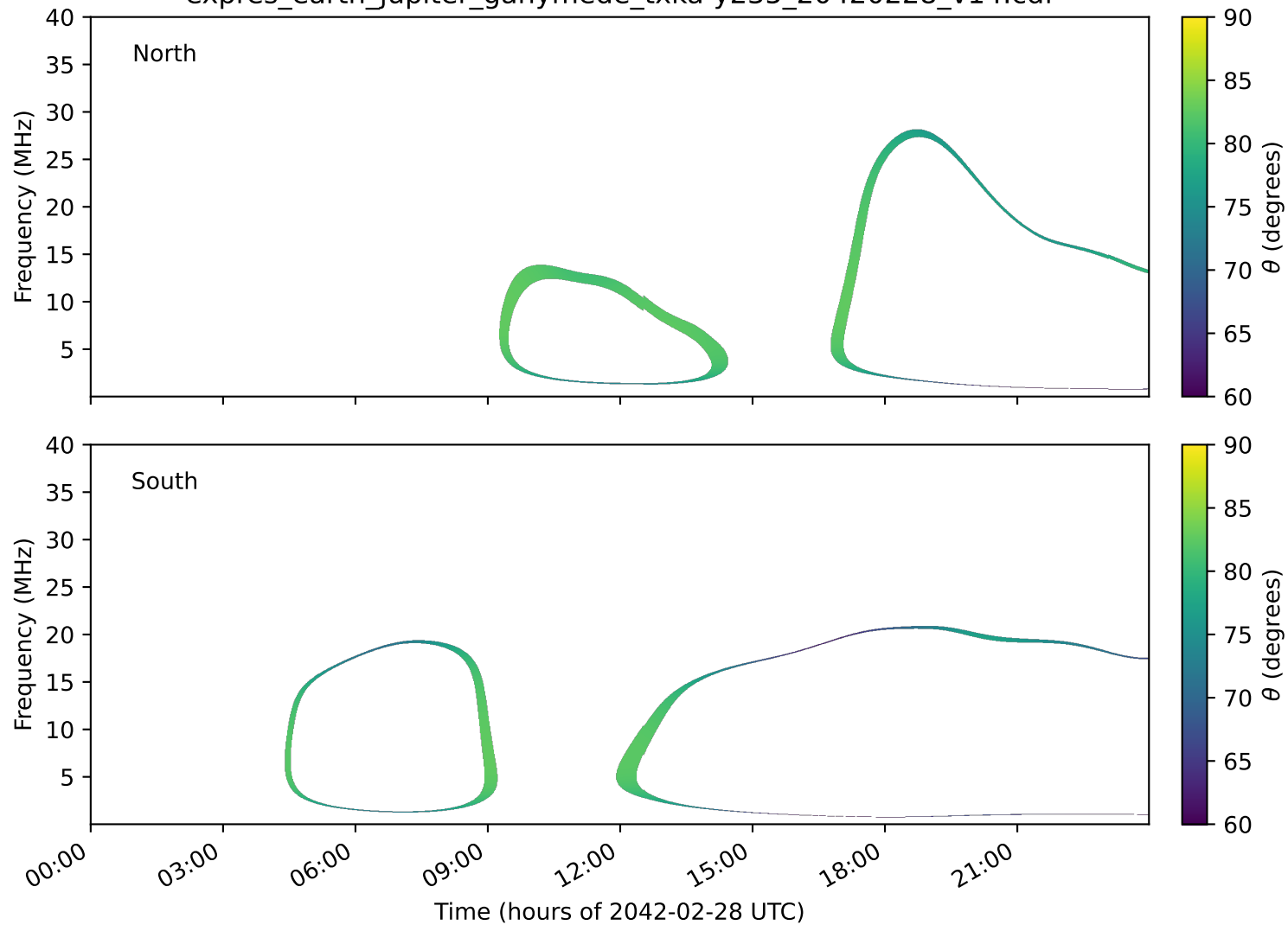
expres_earth_jupiter_ganymede_txka-y235_20420228_v14.cdf
