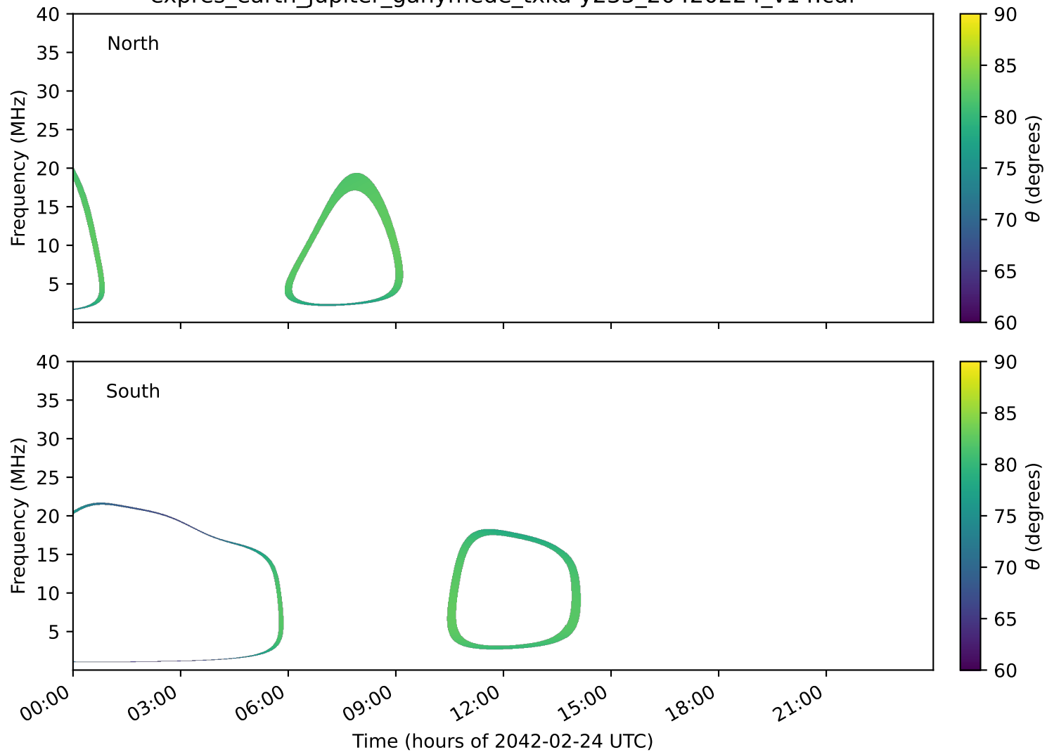
expres_earth_jupiter_ganymede_txka-y235_20420224_v14.cdf
