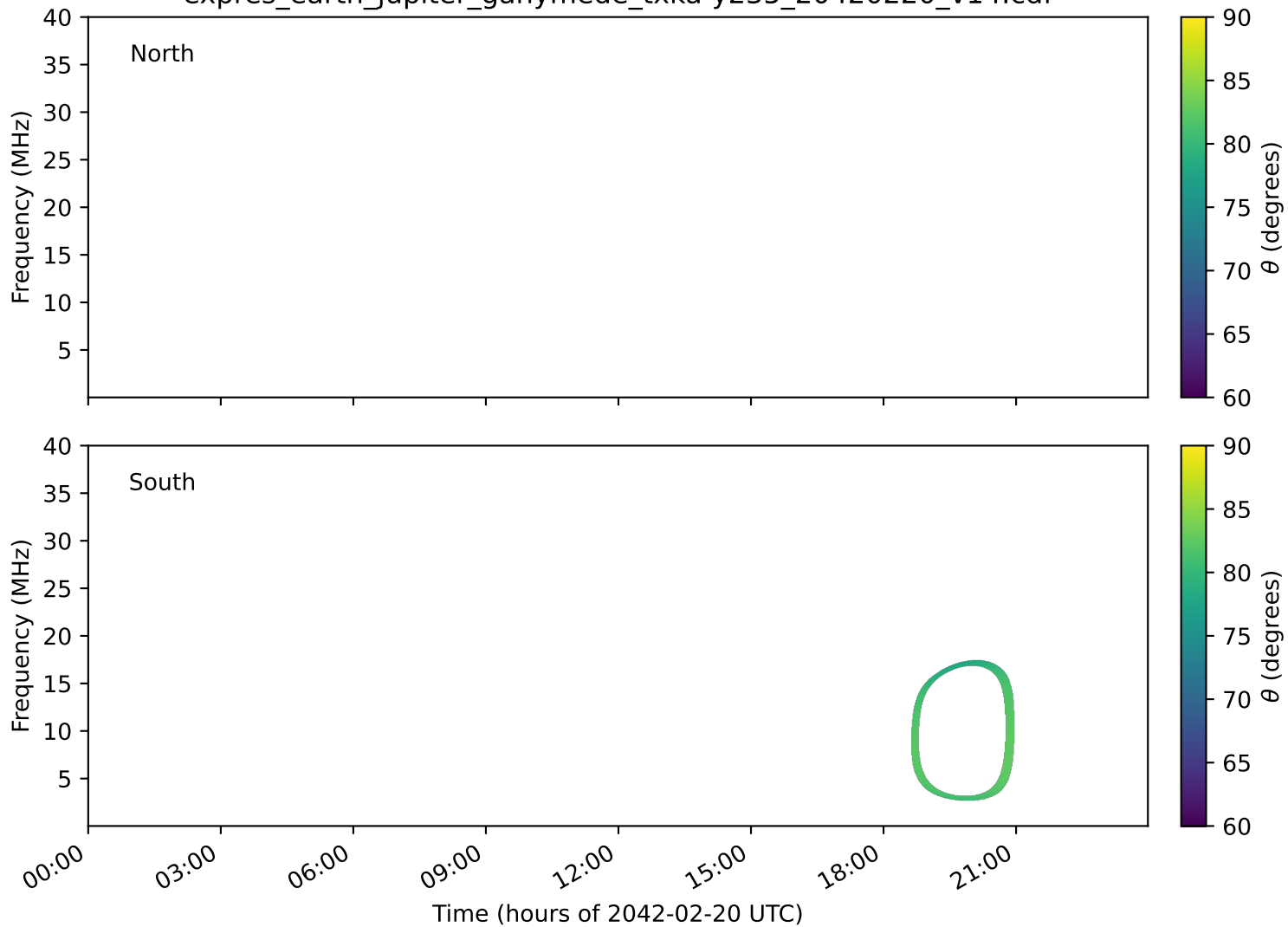
expres_earth_jupiter_ganymede_txka-y235_20420220_v14.cdf
