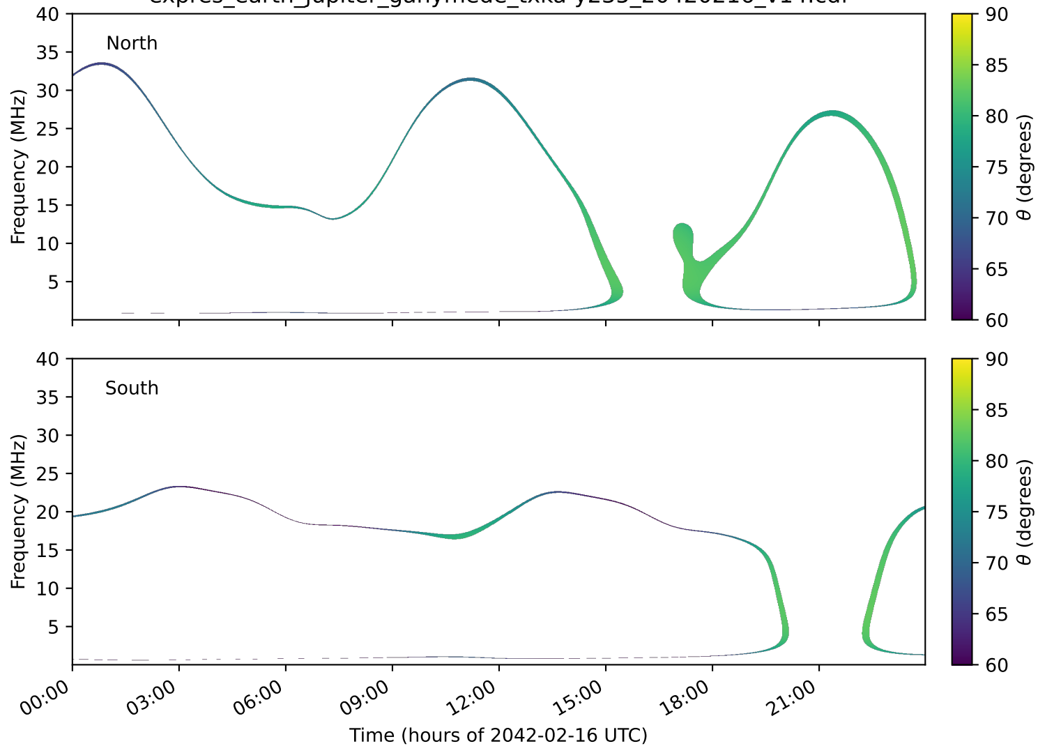
expres_earth_jupiter_ganymede_txka-y235_20420216_v14.cdf
