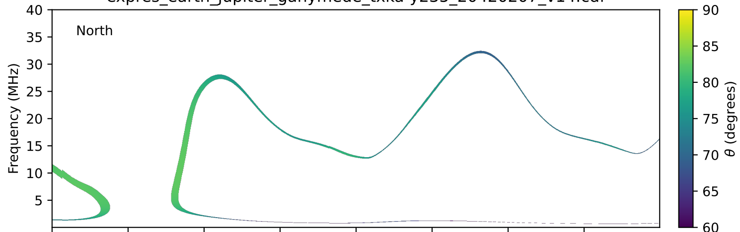
expres_earth_jupiter_ganymede_txka-y235_20420207_v14.cdf
