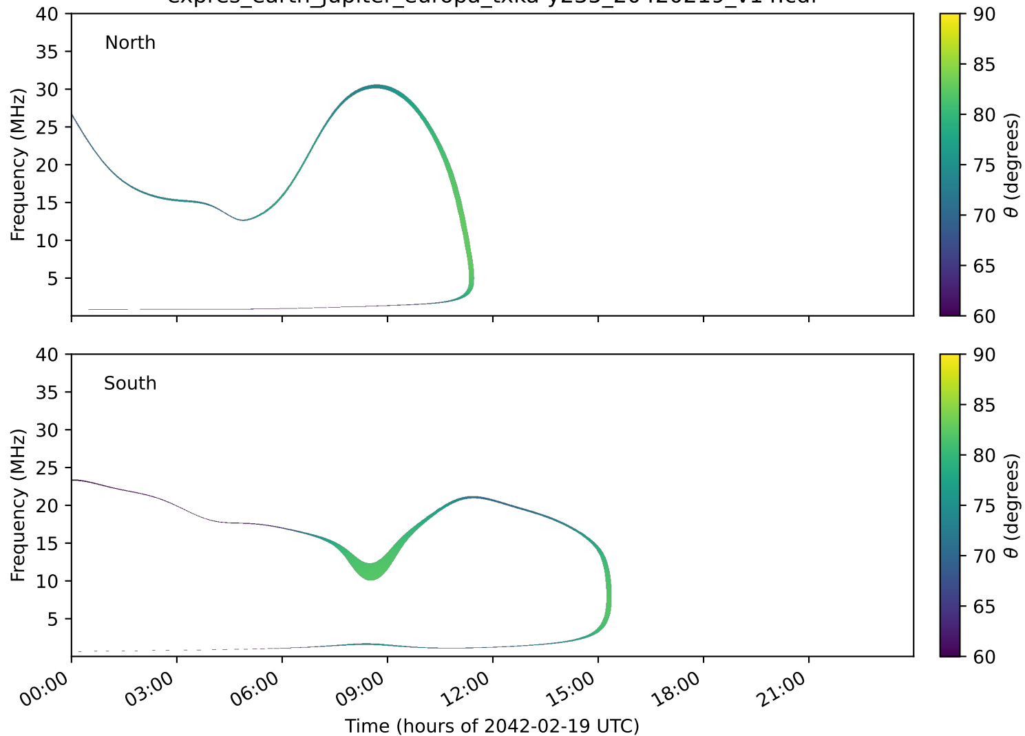
expres_earth_jupiter_europa_txka-y235_20420219_v14.cdf
