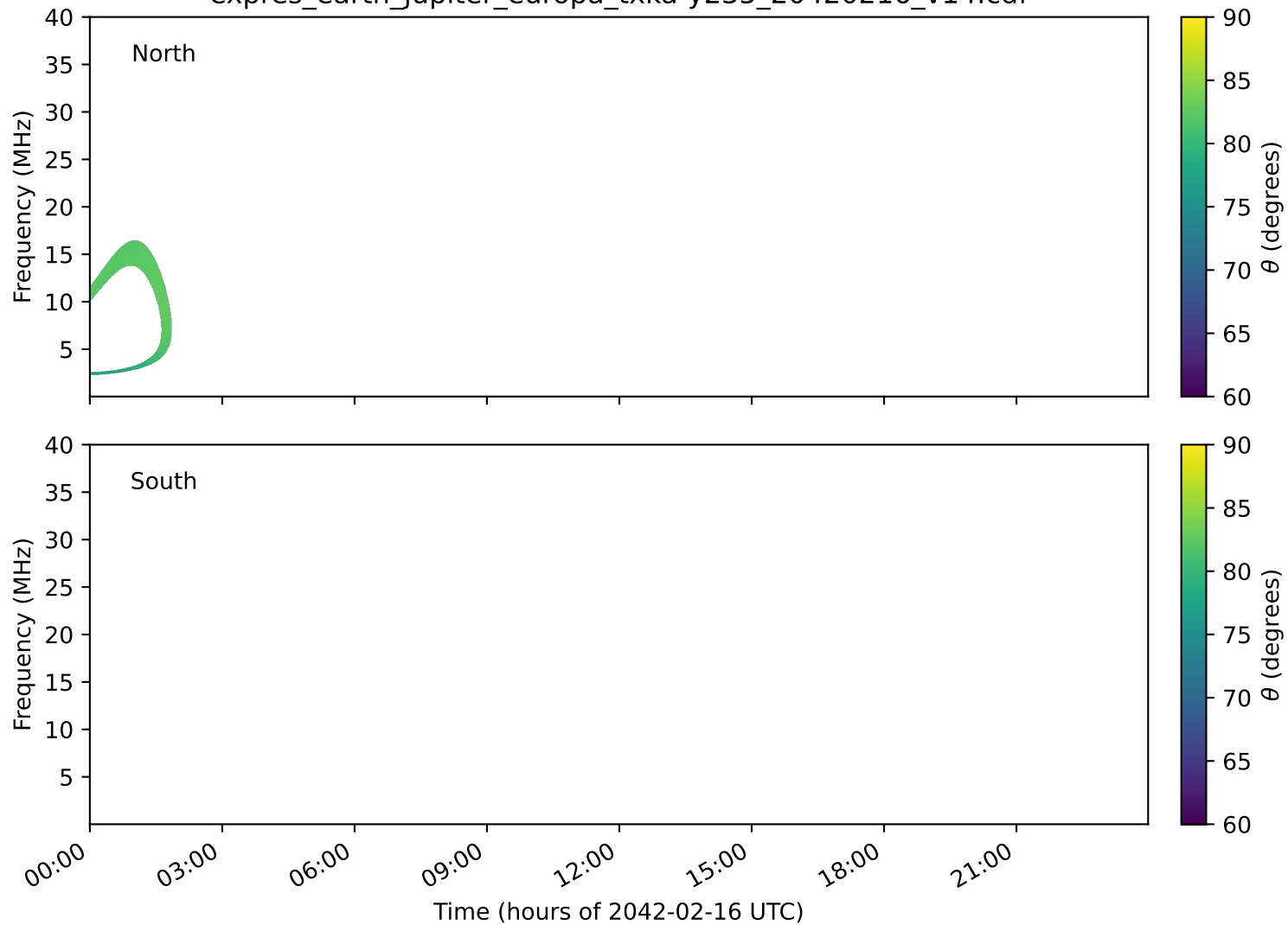
expres_earth_jupiter_europa_txka-y235_20420216_v14.cdf
