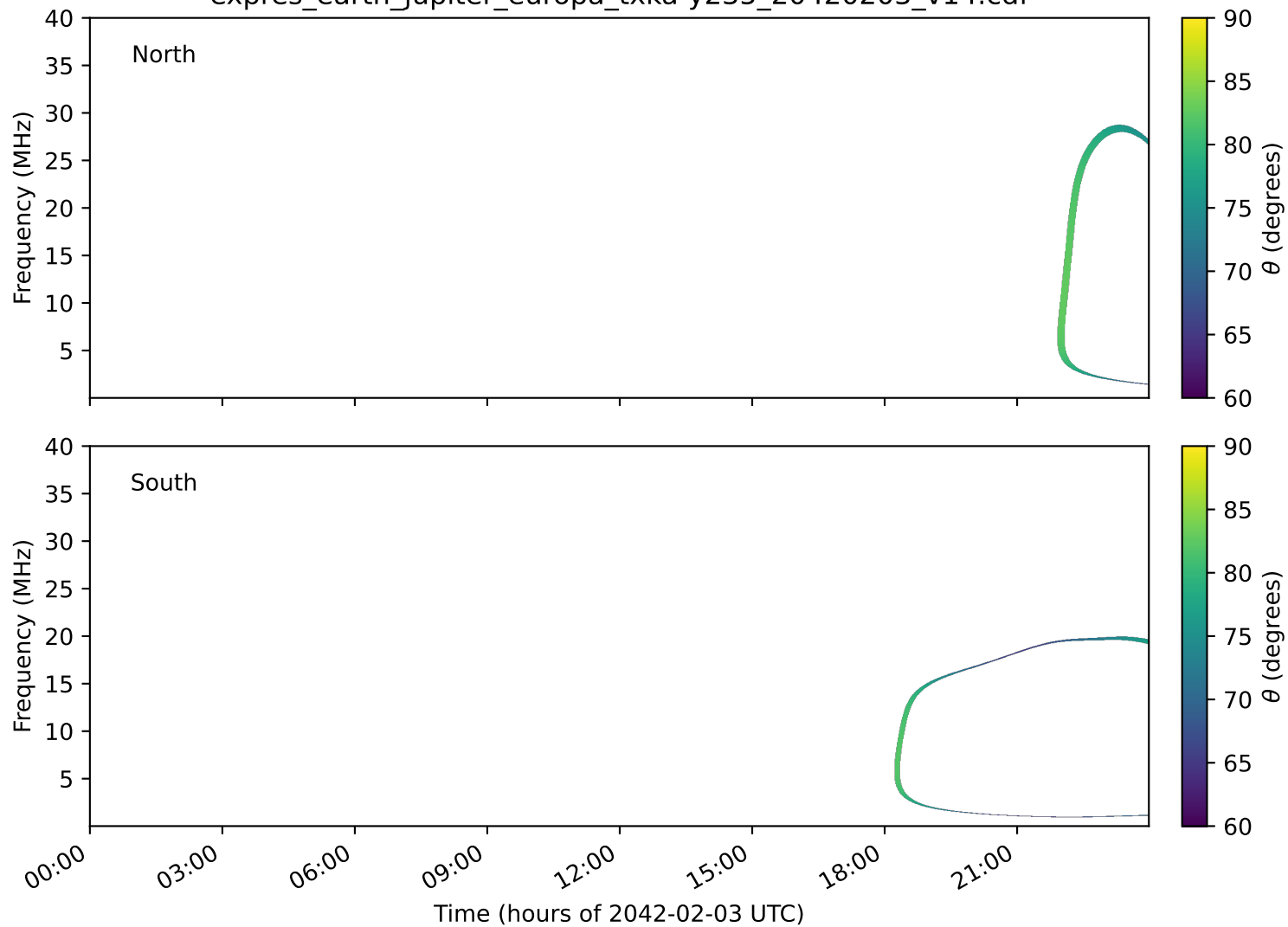
expres_earth_jupiter_europa_txka-y235_20420203_v14.cdf
