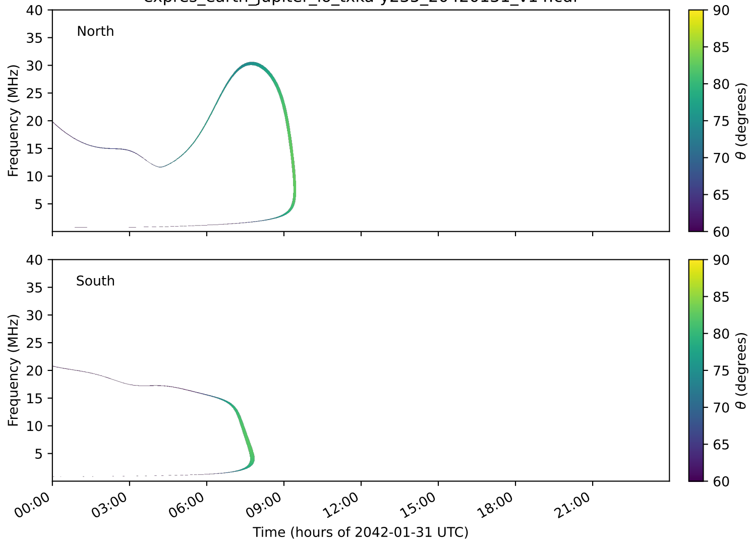
expres_earth_jupiter_io_txka-y235_20420131_v14.cdf
