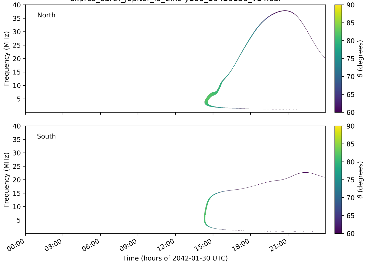
expres_earth_jupiter_io_txka-y235_20420130_v14.cdf
