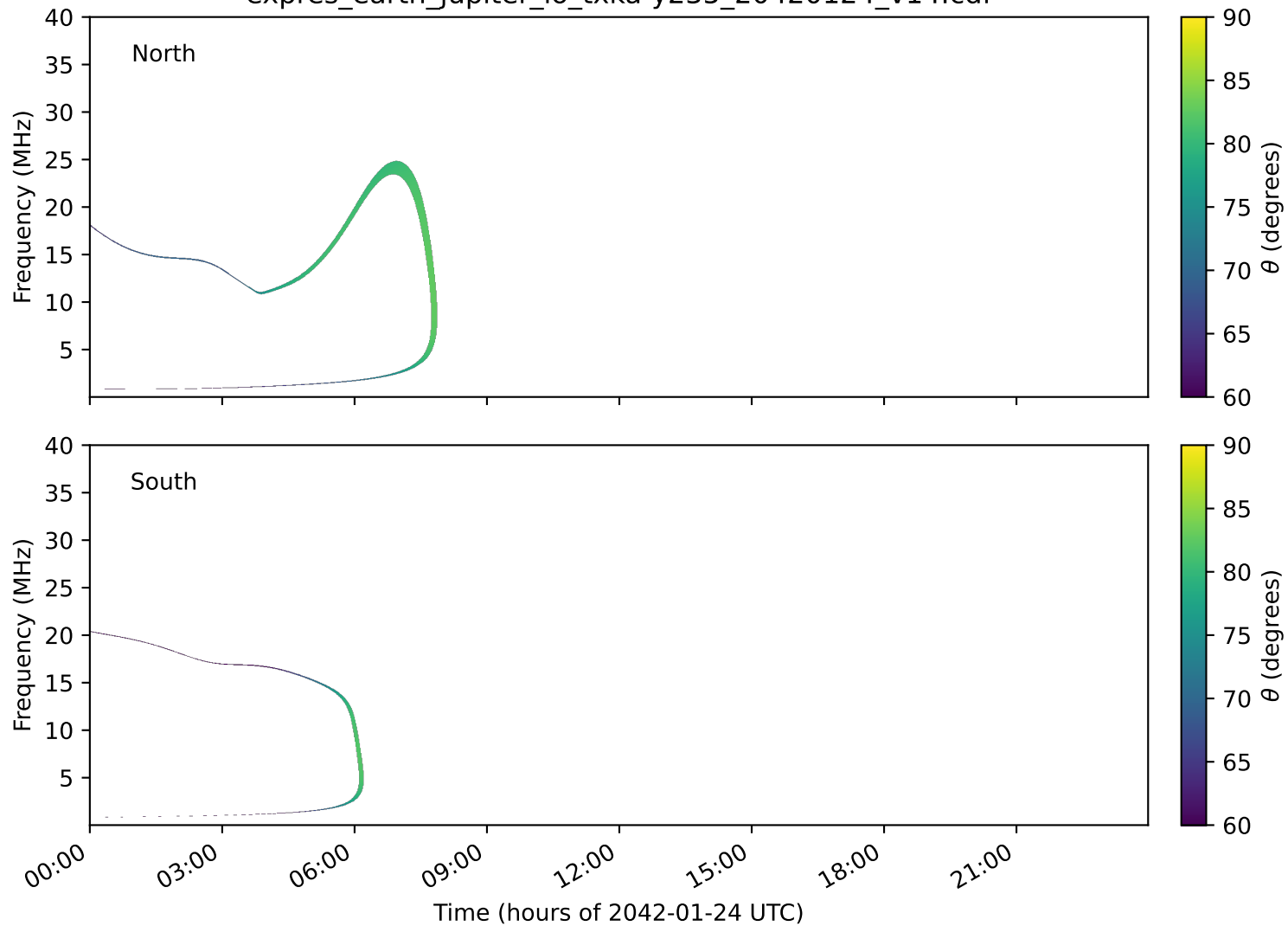
expres_earth_jupiter_io_txka-y235_20420124_v14.cdf
