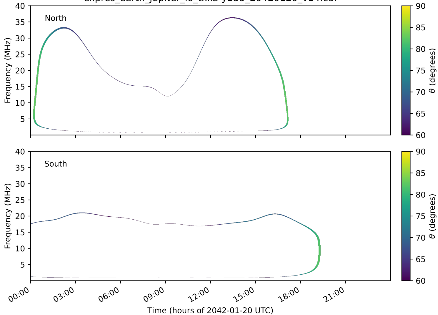
expres_earth_jupiter_io_txka-y235_20420120_v14.cdf
