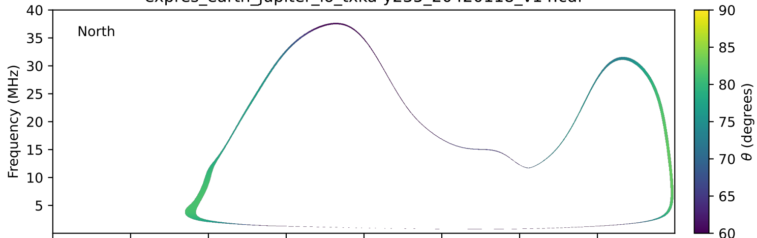
expres_earth_jupiter_io_txka-y235_20420118_v14.cdf
