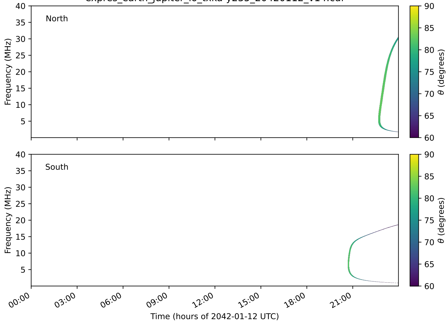
expres_earth_jupiter_io_txka-y235_20420112_v14.cdf
