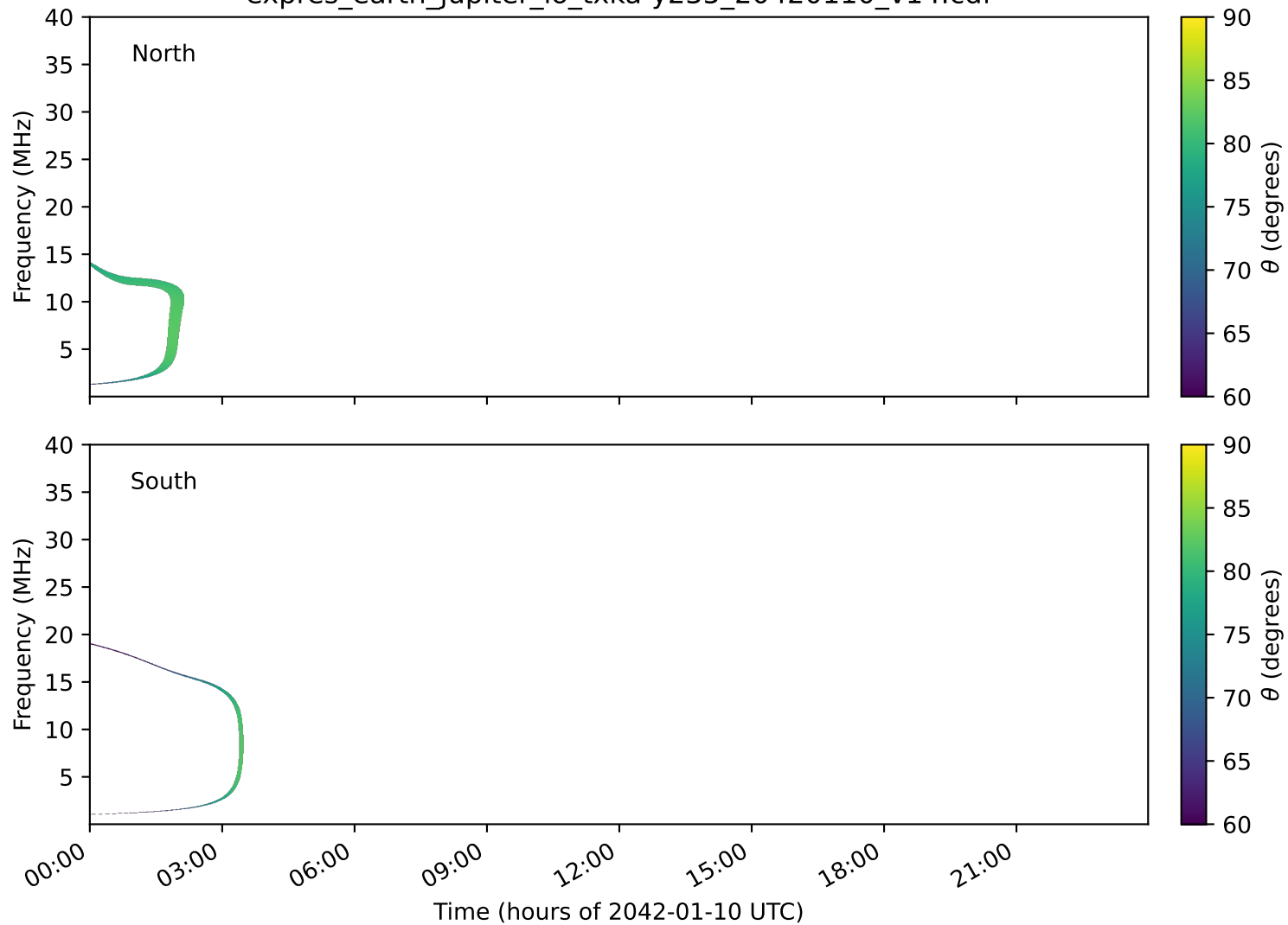
expres_earth_jupiter_io_txka-y235_20420110_v14.cdf
